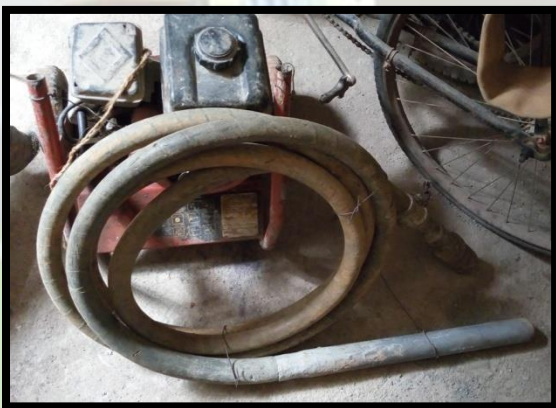
Poker vibrators
